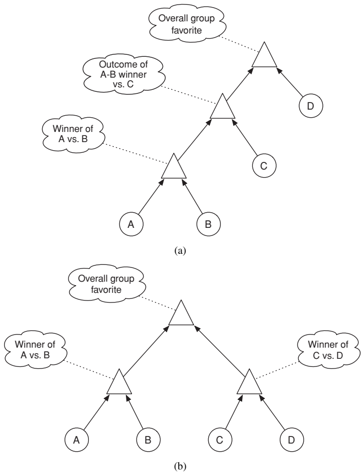
Figure 23.3. One can use majority rule for pairs to build voting systems on three or more alternatives. The alternatives are considered according to a particular “agenda” (in the form of an elimination tournament), and they are eliminated by pairwise majority vote according to this agenda. This produces an eventual winner that serves as the overall group favorite. As shown in (a) and (b), there can be many different orders in which to pair off the alternatives against each other.
