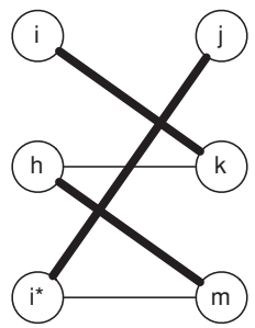
Figure 15.19. The third and final step in analyzing the market with j zeroed out: observe that the rewired preferred-seller graph still contains a perfect matching, in which j is now paired with i^* .
