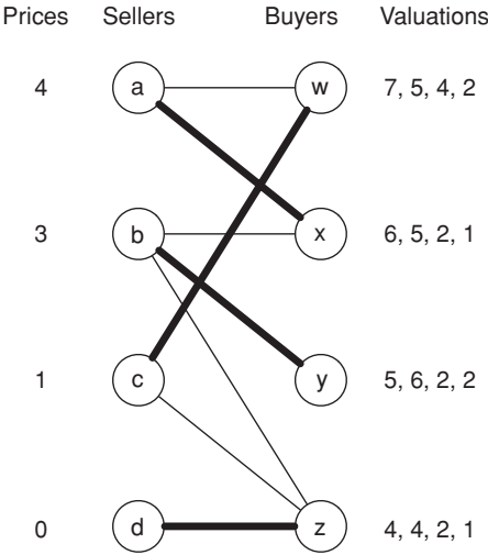
Figure 15.11. A matching market with market-clearing prices of minimum total sum. Note how there is an alternating path from each item, beginning with a nonmatching edge, that leads to the item of zero price.
