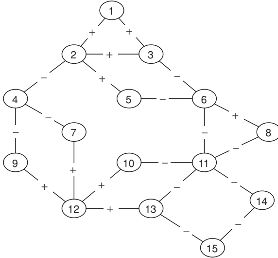
Figure 5.8. In graphs that are not complete, we can still define notions of structural balance when the edges that are present have positive or negative signs, indicating friend or enemy relations, respectively.
