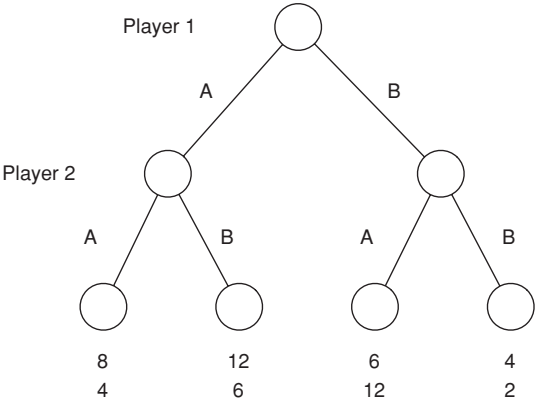
Figure 6.24. A simple game in extensive form.
