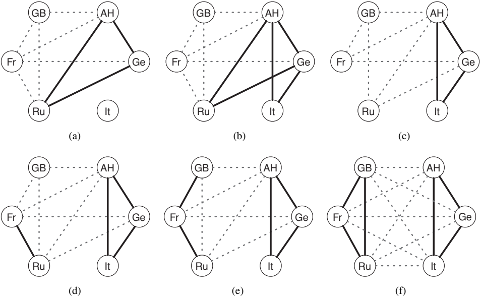
Figure 5.5. The evolution of alliances in Europe, 1872–1907 (the abbreviations GB, Fr, Ru, It, Ge, and AH stand for Great Britain, France, Russia, Italy, Germany, and Austria-Hungary, respectively): (a) Three Emperors’ League, 1872–1881; (b) Triple Alliance, 1882; (c) German–Russian Lapse, 1890; (d) French–Russian Alliance, 1891–1904; (e) Entente Cordiale, 1904; (f) British Russian Alliance, 1907. Solid dark edges indicate friendship while dotted edges indicate enmity. Note how the network slides into a balanced labeling – and into World War I. (This figure and example are from Antal et al. [20] and Elsevier Science and Technology Journals.)
