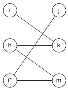
Figure 15.18. The second step in analyzing the market with j zeroed out: build the new preferred-seller graph by rewiring j 's preferred-seller edges to point to the zero-priced items.
