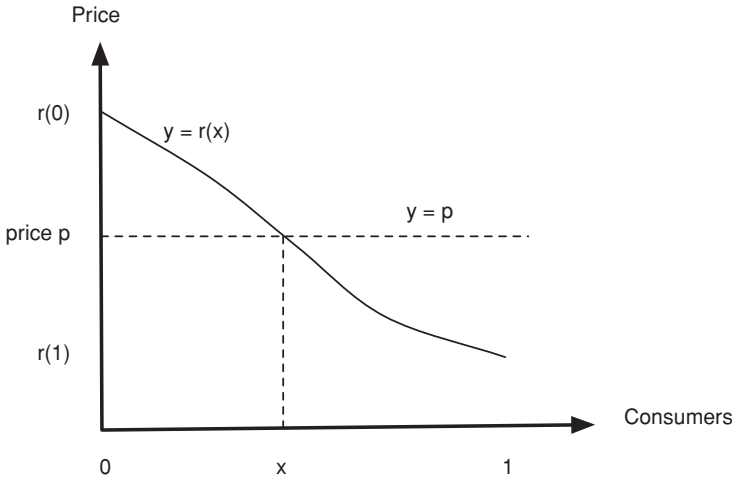
Figure 17.1. When there are no network effects, the demand for a product at a fixed market price p can be found by locating the point where the curve y = r(x) intersects the horizontal line y = p .
