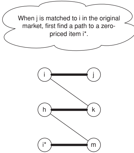
Figure 15.17. The first step in analyzing the market with j zeroed out: find an alternating path from item i – to which buyer j was matched in the original market – to a zero-priced item i^* .
