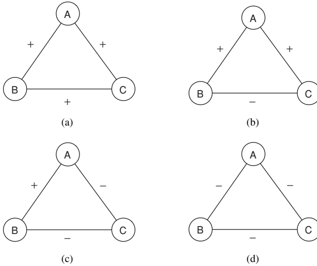
Figure 5.1. Structural balance: each labeled triangle must have one or three positive edges. (a) A, B, and C are mutual friends: balanced. (b) A is friends with B and C, but they don't get along with each other: not balanced. (c) A and B are friends and C is a mutual enemy: balanced. (d) A, B, and C are mutual enemies: not balanced.
