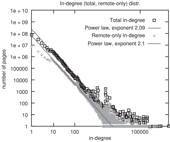
Figure 18.2. A power-law distribution (such as this one for the number of Web page in-links, from Broder et al. [80]) shows up as a straight line on a log-log plot. (Courtesy of Elsevier Limited.)
