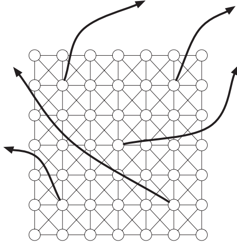
Figure 20.3. The general conclusions of the Watts–Strogatz model still follow even if only a small fraction of the nodes on the grid each have a single random link.
